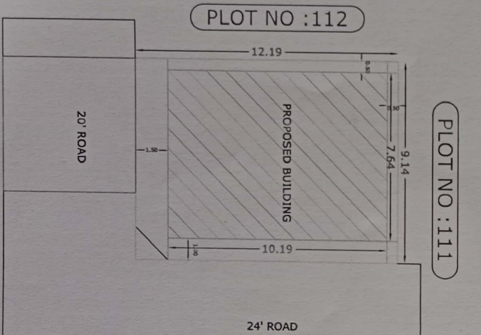
SITE PLAN
