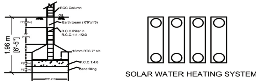
FOUNDATION DETAILS
