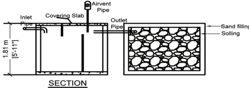
SECTION
