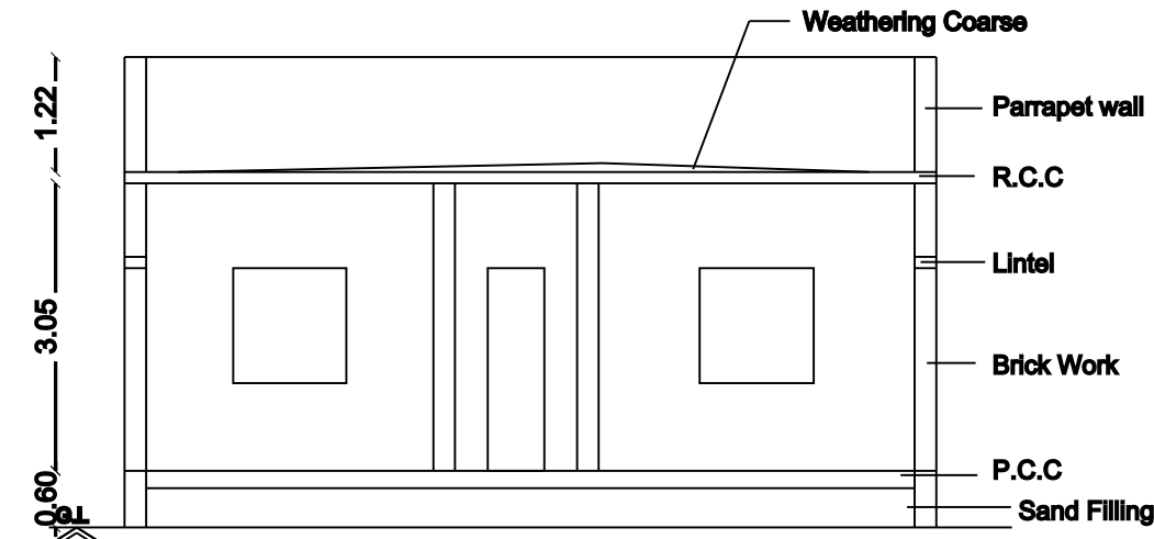
SECTION ON-A'A
