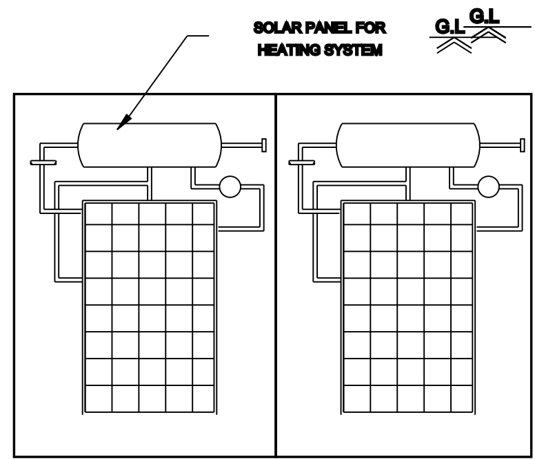
SOLAR HEATING SYSTEM
