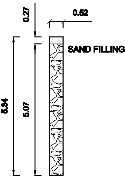
DETAILS OF PERCULATION PIT
