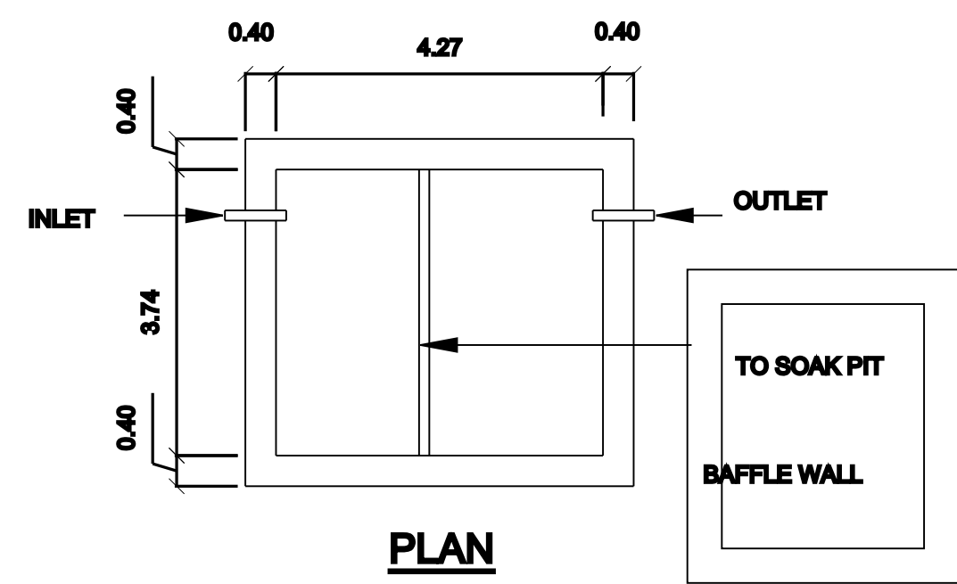
SEPTIC. TANK
