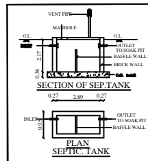
PLAN SEPTIC TANK
