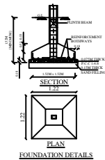
FOUNDATION DETAILS
