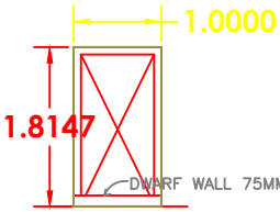
WICKET GATE
