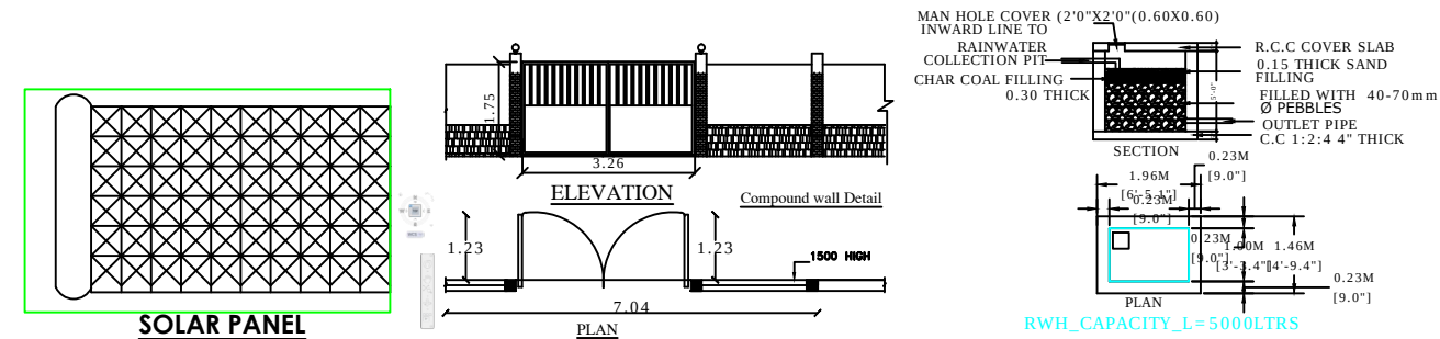
PLAN
