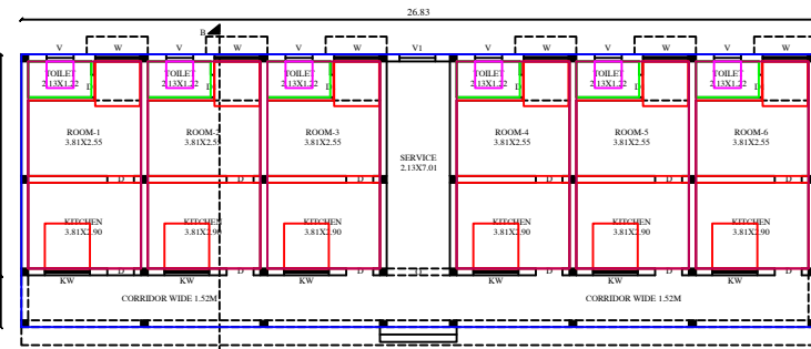
PRO. GROUND FLOOR PLAN
