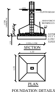
FOUNDATION DETAILS
