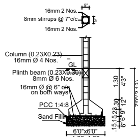
FOUNDATION DETAIL
