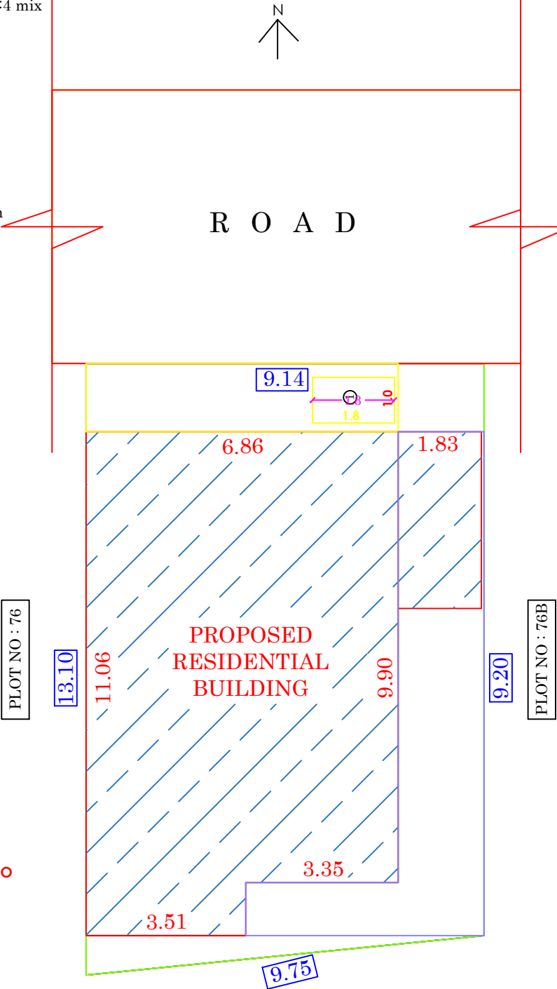
SITE PLAN
