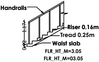
STAIRCASE DETAILS
