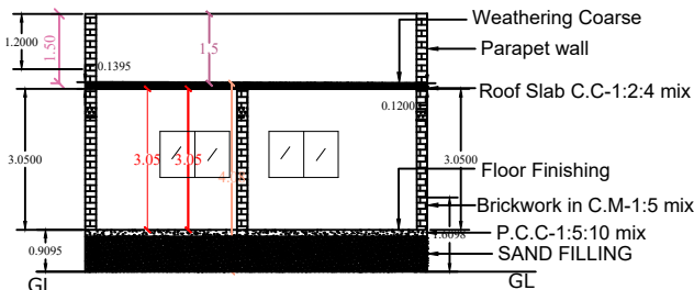
CROSS SECTION ON AB
