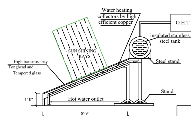
SECTION SOLAR WATER HEATER
