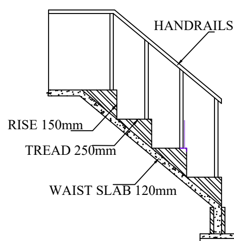
STAIRCASE DETAILS
