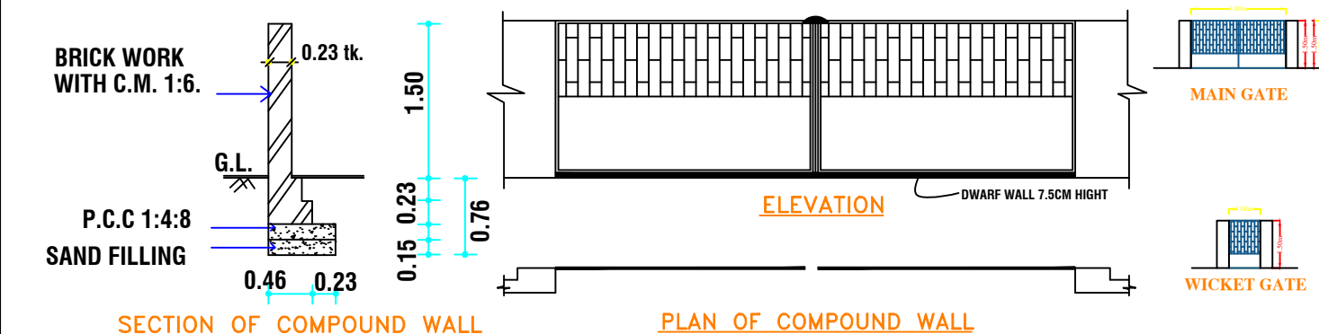
SECTION OF COMPOUND WALL
