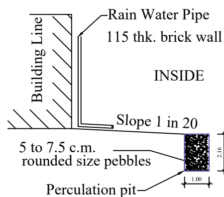
RAIN WATER HARVESTING PERCUATION PIT RW_H_CAPACITY_L=2000LTRS
