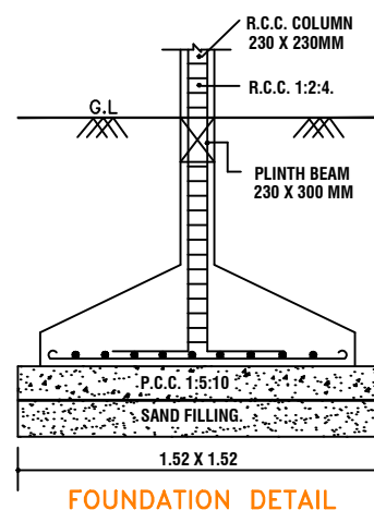
FOUNDATION DETAIL
