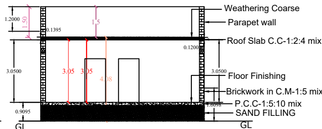
CROSS SECTION ON AB
