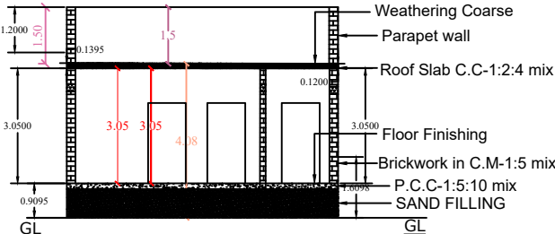
CROSS SECTION ON AB
