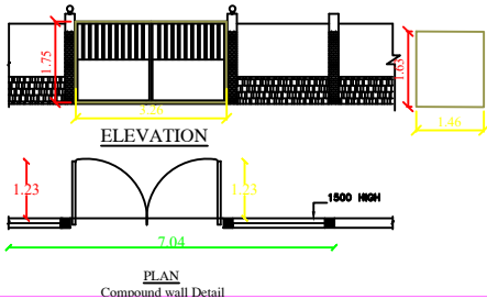
PLAN Compound wall Detail
