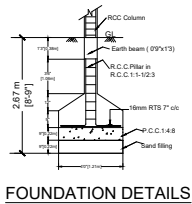
FOUNDATION DETAILS
