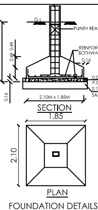
FOUNDATION DETAILS
