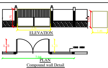
Compound wall Detail
