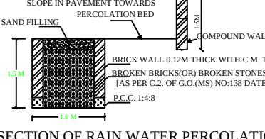
SECTION OF RAIN WATER PERCOLATION BED
