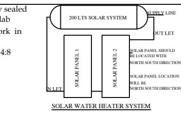
SOLAR WATER HEATER SYSTEM
