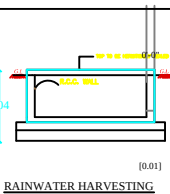
RAINWATER HARVESTING
