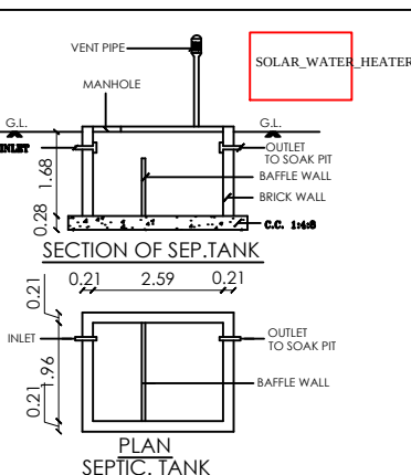
PLAN SEPTIC TANK
