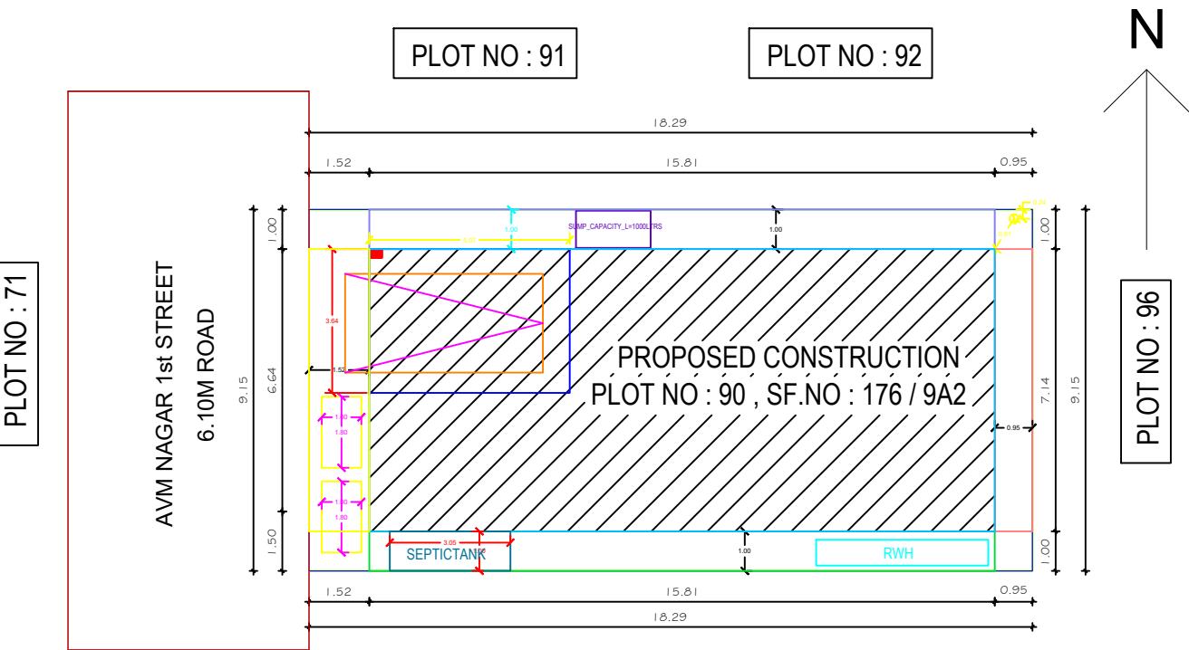
SITE PLAN
