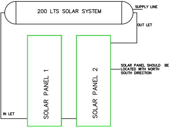
SOLAR WATER HEATER SYSTEM
