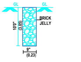
PERCULATION PIT
