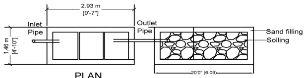
DETAILS OF SEPTIC TANK & DISPERSION TRENCH
