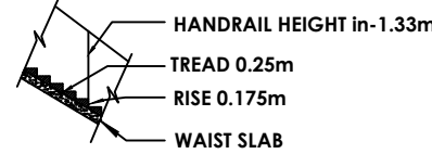
STAIRCASE DETAILS
