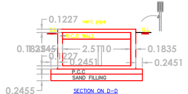
SECTION ON D-D
