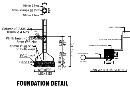
FOUNDATION DETAIL
