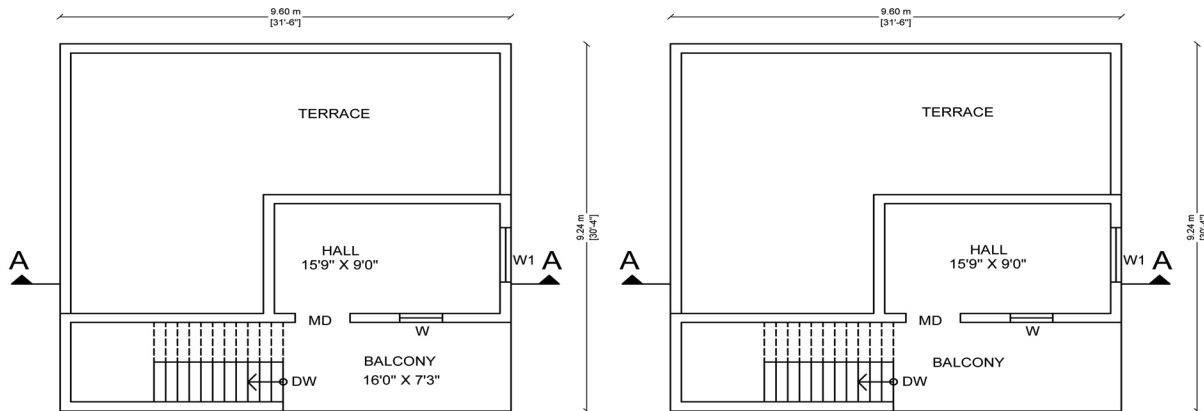
FIRST FLOOR
