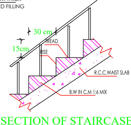
SECTION OF STAIRCASE
