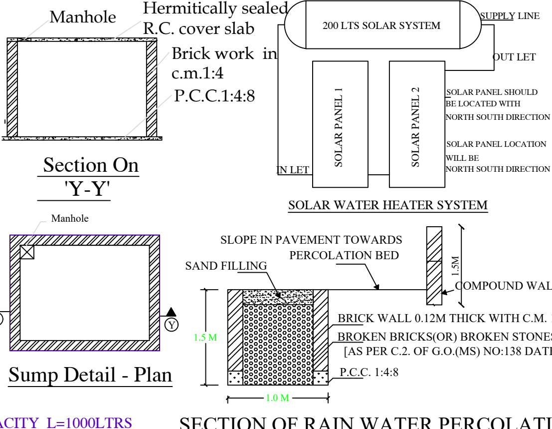
SECTION OF RAIN WATER PERCOLATION BED
