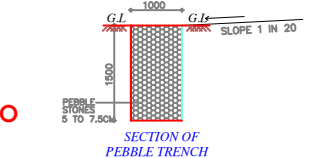
SECTION OF PEBBLE TRENCH
