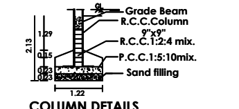
COLUMN DETAILS
