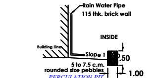
RAIN WATER PIPE
