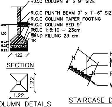
COLUMN DETAILS
