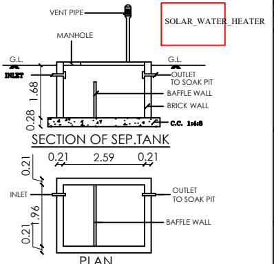
PLAN SEPTIC TANK
