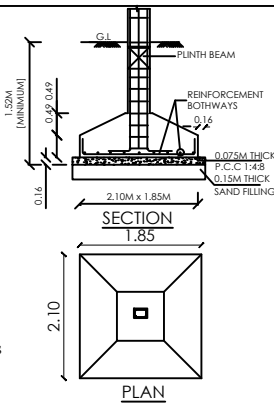
FOUNDATION DETAILS
