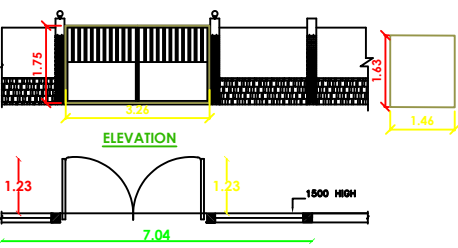
COMPOUND WALL DETAILS
