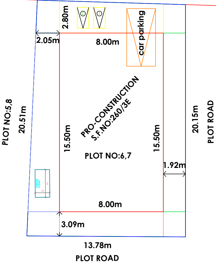
SITE PLAN-SCALE1:100
