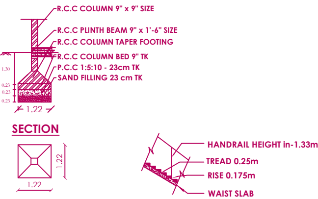
COLUMN DETAILS PLAN
