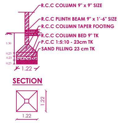
COLUMN DETAILS PLAN
