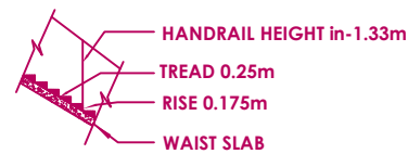
STAIRCASE DETAILS
