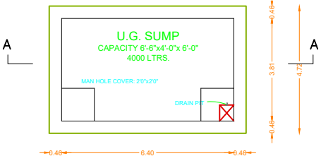
SUMP DETAIL SCALE 1"=4'0"
