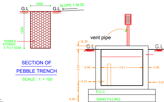
SECTION ON D-D
