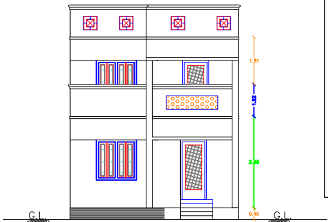
FRONT ELEVATION
