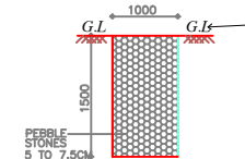
SECTION OF PEBBLE TRENCH
