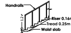
STAIRCASE DETAILS
