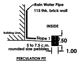
PERCOLATION PIT
