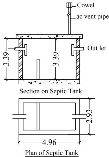
Plan of Septic Tank
