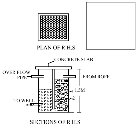
SECTIONS OF R.H.S.
