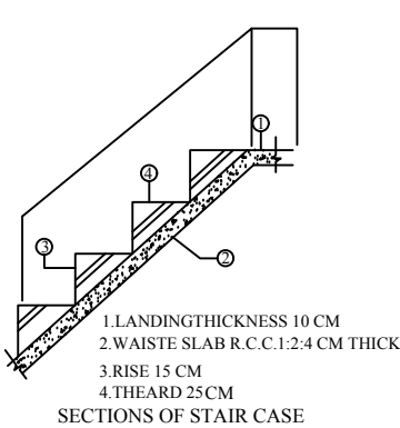
SECTIONS OF STAIR CASE
