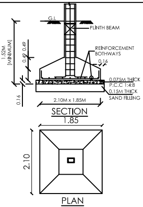
FOUNDATION DETAILS
