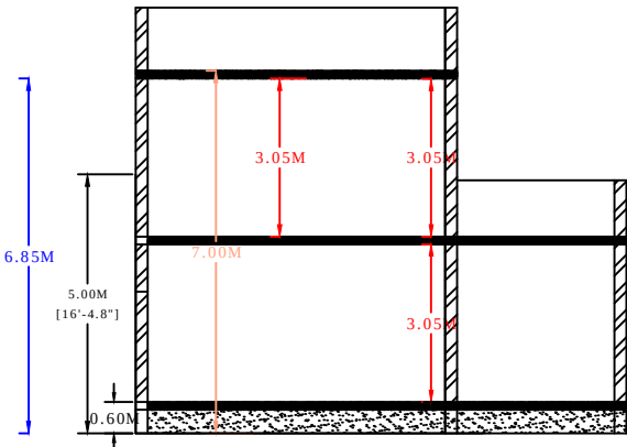
SECTION ON XX
