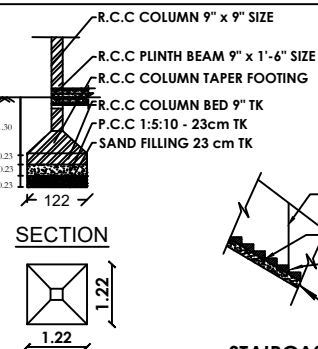
COLUMN DETAILS PLAN
