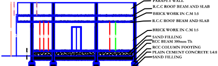
SECTION "AB"
