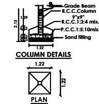
COLUMN DETAILS
