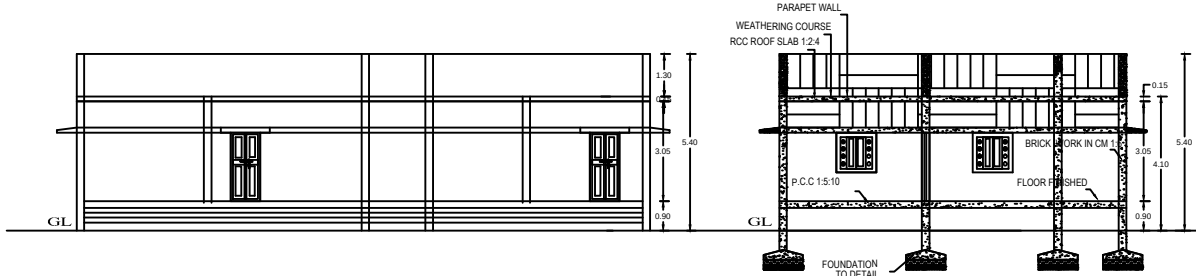
FRONT ELEVATION.
