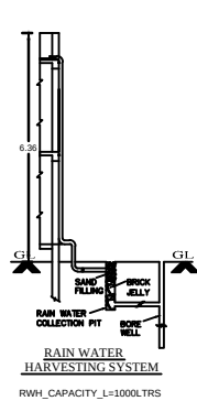
RAIN WATER HARVESTING SYSTEM RWH_CAPACITY_L=1000LTRS
