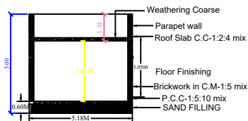
CROSS SECTION ON XX
