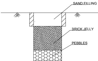
RAIN WATER HARVESTING SYSTEM (NOT TO SCALE)
