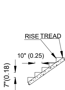
SECTION ON STAIRCASE (NOT TO SCALE)
