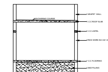
SECTION ON A-A
