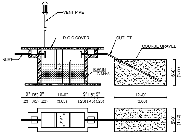
SEPTIC TANK & D-TRENCH DETAILS (NOT TO SCALE)
