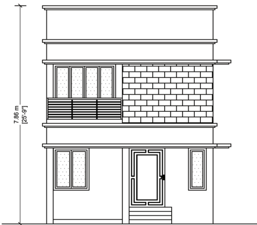
FRONT ELEVATION
