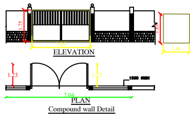
Compound wall Detail
