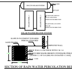
SECTION OF RAIN WATER PERCOLATION BED
