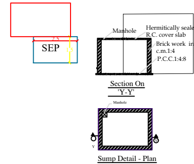
Sump Detail - Plan
