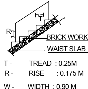
STAIRCASE DETAILS (NOT TO SCALE )
