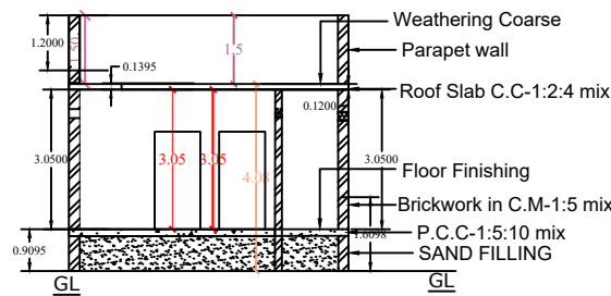
CROSS SECTION ON AB
