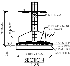
FOUNDATION DETAILS
