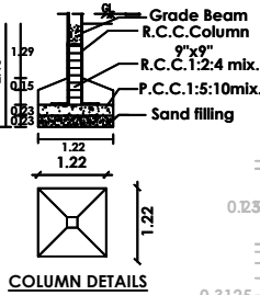
COLUMN DETAILS
