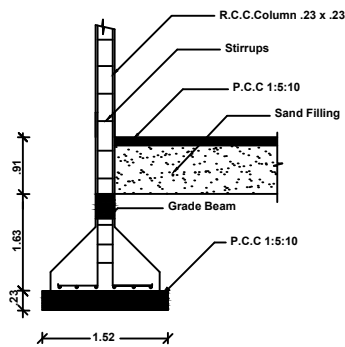
COLUMN DETAIL
