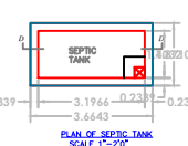
PLAN OF SEPTIC TANK
