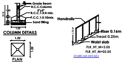
STAIRCASE DETAILS
