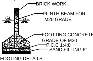
FOOTING DETAILS
