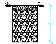
RWH SECTION
