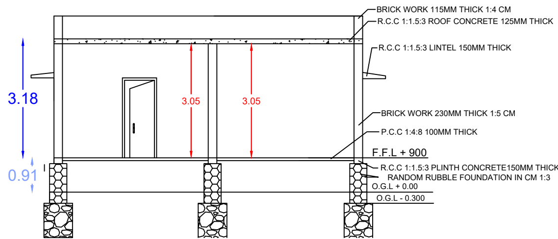
SECTIONAL ELEVATION 'A-B'
