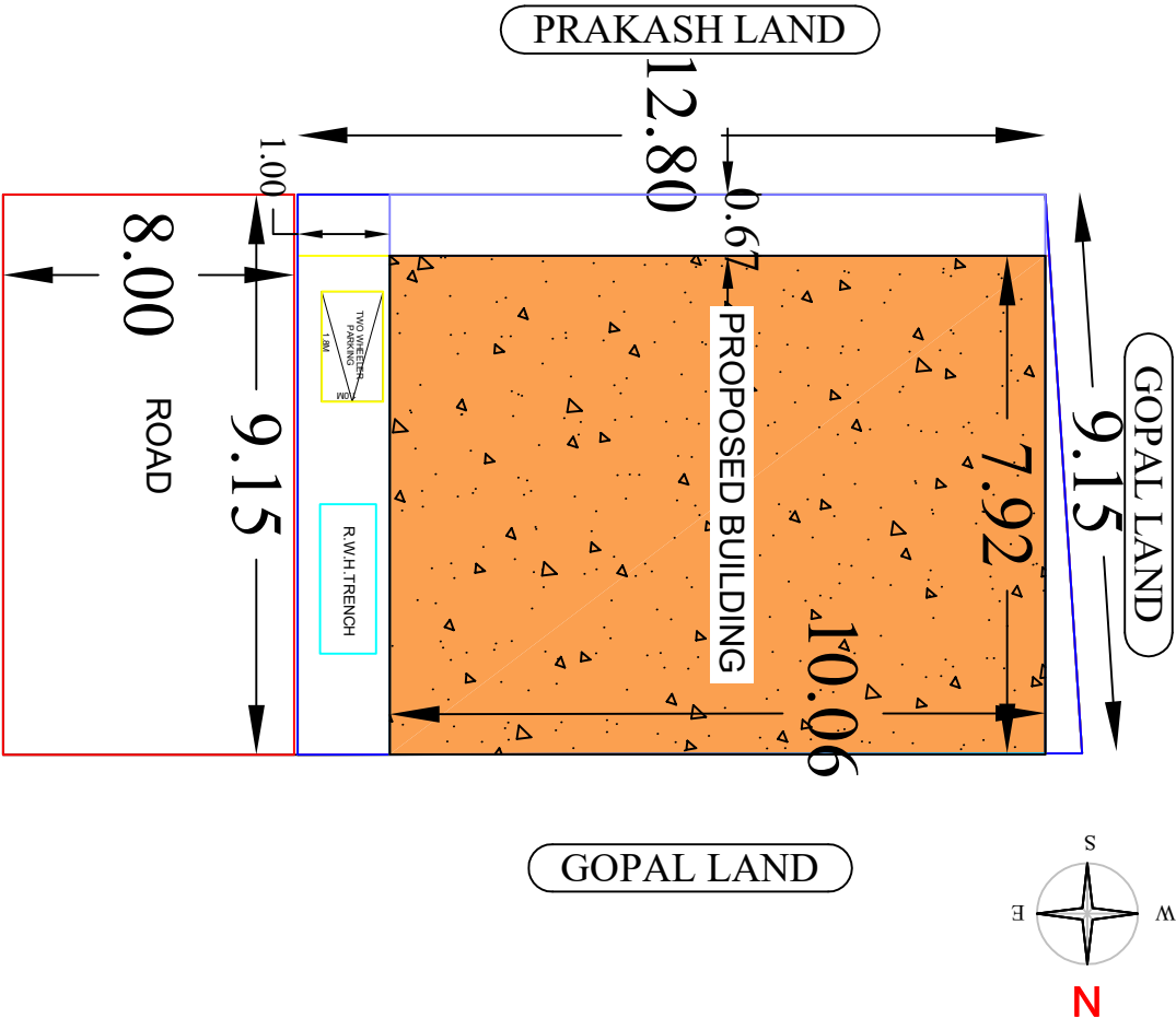
SITE PLAN
