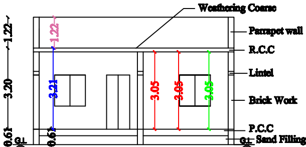
SECTION ON-A'A'
